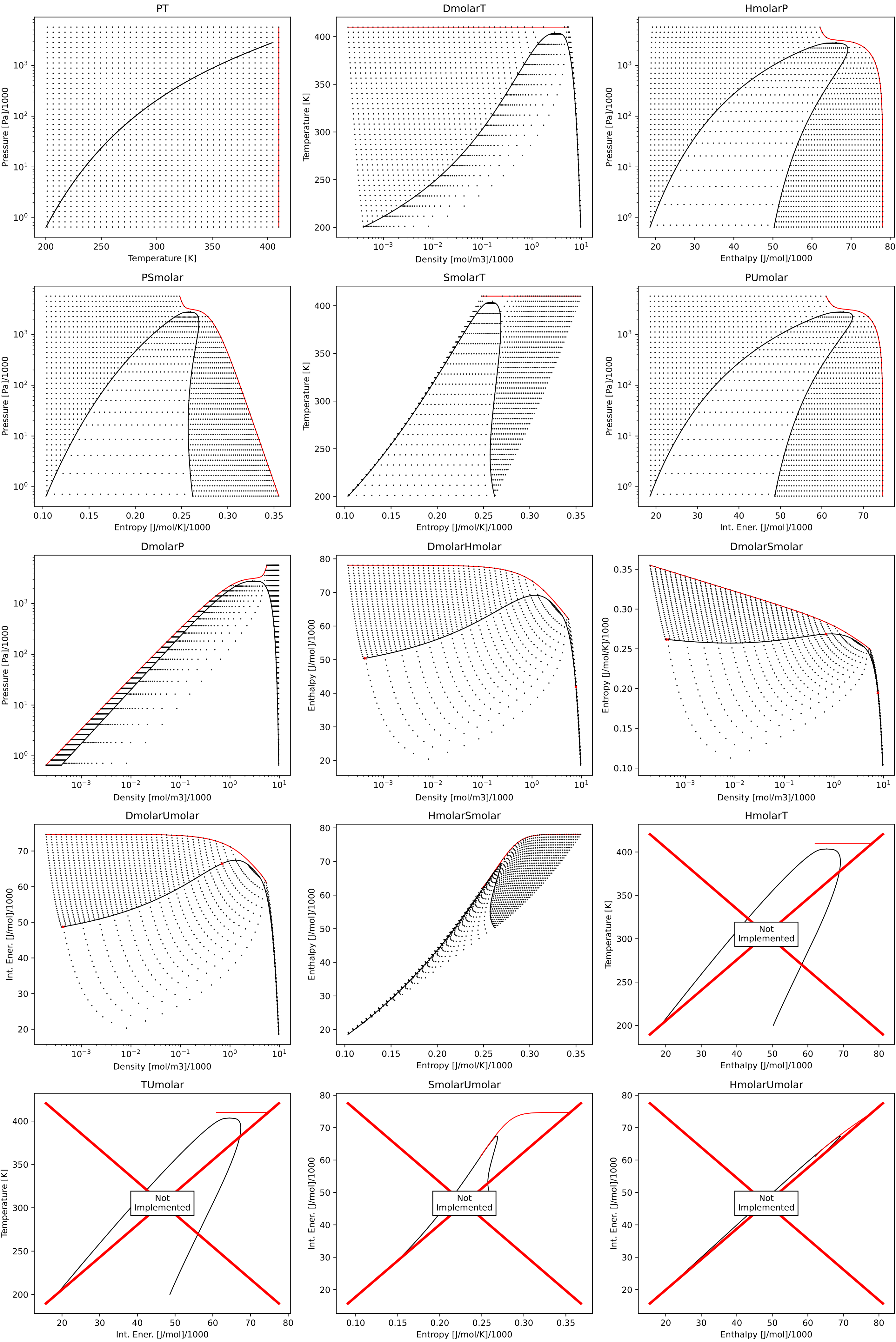
Consistency plots for R1336mzz(E)
